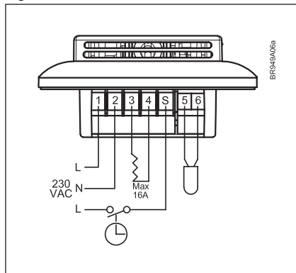
Night setback
